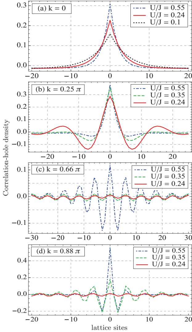
FIG. 2. (Color online) Correlation-hole density in the vicinity of the impurity located at 0 for (a) k = 0 , (b) k = 0.25\pi , (c) k = 0.66\pi , and (d) k = 0.88\pi , from our variational wave function. At strong interactions, we see polaronic excitation for all values of k . Here the impurity displaces nearby bath atoms, creating a (symmetric) bath density oscillation of period \approx 4\pi/k within the healing length. The healing length increases with decreasing U/J and is largest for k \approx 2\pi/3 . For nonzero k , the system crosses over to the particle-hole continuum below a certain interaction strength, where the bath distribution becomes essentially independent of the impurity location. This crossover occurs at U/J \approx 0.16, 0.44, and 0.29 for k = 0.25\pi, 0.66\pi, and 0.88\pi , respectively. Such a crossover does not happen for k = 0 (compare with Fig. 1).
