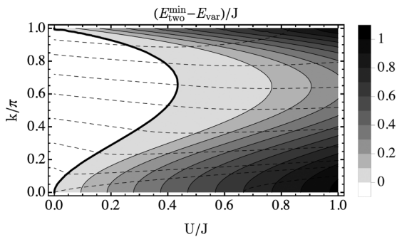
FIG. 5. Contour plot of the energy difference between our variational state in Eq. (13) and the bottom of the uncorrelated particle-hole continuum of states from Eq. (15). Dotted lines show constant energy contours for E_{\text{var}} . For U/J \gtrsim 0.44 , the variational ground state is lower in energy and describes a stable polaron. The two energies coincide to the left of the dark contour. Thus at weaker interactions there exists a growing range of momenta where the polaron is unstable, and the ground state belongs to the particle-hole continuum.
