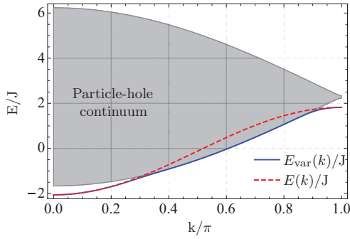
FIG. 4. (Color online) Energy of states with one impurity and one excess hole for U/J = 0.37 . Solid line denotes the variational ground state, E_{\text{var}}(k) ; shaded region denotes the independent particle-hole continuum; dashed line denotes the approximate polaron dispersion E(k) = E_0 - 2J_{\text{eff}} \cos(k) , where E_0 and J_{\text{eff}} are chosen so that E(0) = E_{\text{var}}(0) and E(\pi) = E_{\text{var}}(\pi) . At small and large k , E_{\text{var}}(k) describes a stable polaron. For intermediate k , the polaron energy lies within the particle-hole continuum. Thus we expect it to be short lived due to Landau damping.
