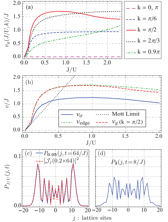
FIG. 3. (Color online) (a) Polaron group velocity at different momenta. After a rapid growth for small J/U , these saturate for J/U \gtrsim 0.5 . (b) Propagation speed of an initially localized impurity in |\psi(0)\rangle = \hat{b}_{0,\uparrow}\hat{b}_{0,\downarrow}^\dagger|\text{MF}\rangle projected into our variational subspace. v_\sigma and v_{\text{edge}} denote expansion speeds of the standard deviation and the leading edges of the impurity distribution, respectively. v_{\text{edge}} closely mimics the group velocity at k = \pi/2 . For J/U \gtrsim 0.5 , both speeds level off at values much smaller than the free-particle tunneling 2J . (c, d) Impurity distribution for J/U = 0.05 and 2 , respectively. In the Mott phase the distribution is described by a squared Bessel function, as predicted by the Heisenberg model, whereas for large J/U it has a distinctly different shape.
