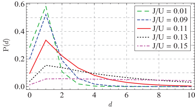
FIG. 7. (Color online) Separation probability of the two impurities, as predicted by the variational wave function in Eq. (16) on a lattice with 40 sites. In the Mott and the strongly interacting superfluid phase, the most probable separation of the impurities is one site, and the probabilities fall roughly exponentially with distance. For weaker interactions, the probabilities do not decay.
