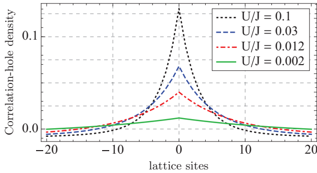
FIG. 1. (Color online) Correlation-hole density in the Bogoliubov approximation for zero total momentum, plotted with \mathcal{N} = 101 . The impurity-hole binding weakens at lower U/J , leading to a flatter profile.
