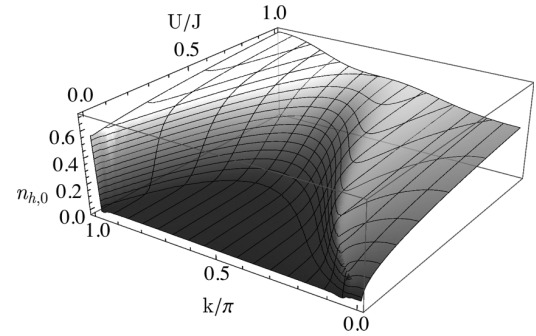
FIG. 6. Correlation-hole density at the impurity site. As the system crosses over from the polaronic to the two-particle regime, the hole density rapidly falls toward zero. These correlations can be measured in experiments.
